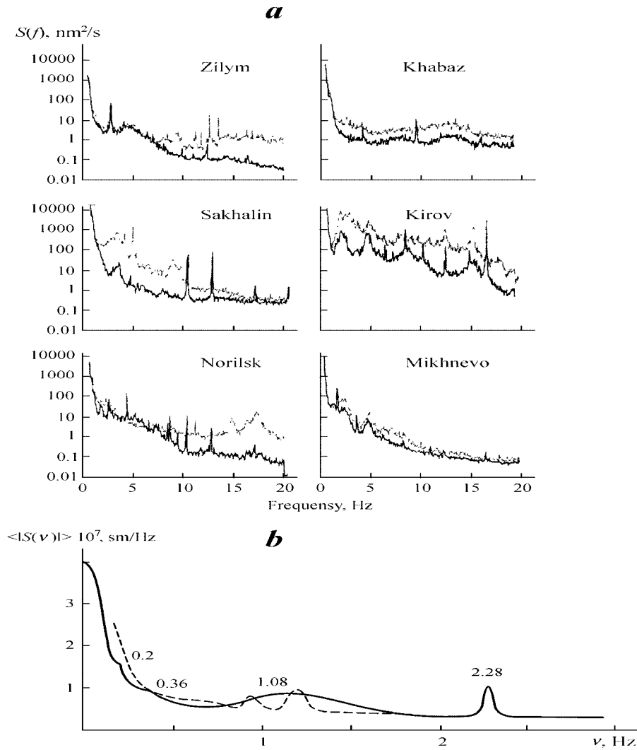
Fig. 1 a, b. Examples of spectral presentation for seismic noises.
